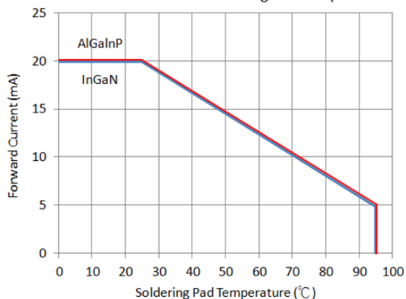
Forward Current vs. Soldering Pad Temperature
